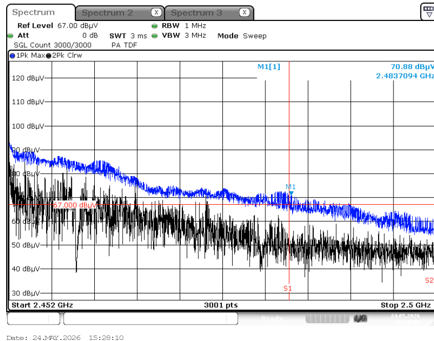
Radiated Restricted Band Edges plot – Peak Result (802.11n(HT20)_ MCS0, Ch.7, X-H)
