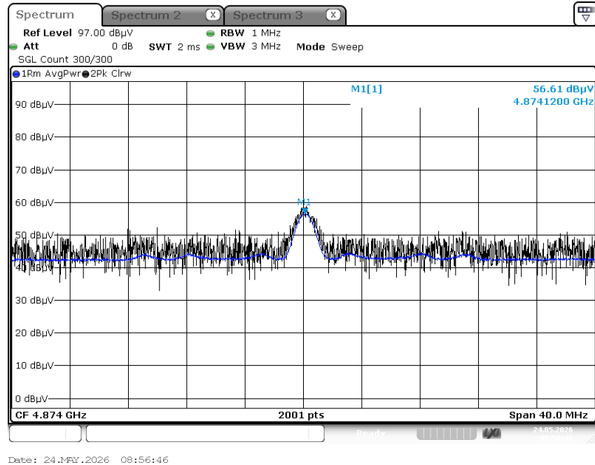
Radiated Spurious Emissions plot – Average Result (802.11b_1 Mbps, Ch.6 2nd Harmonic, Y-H)
