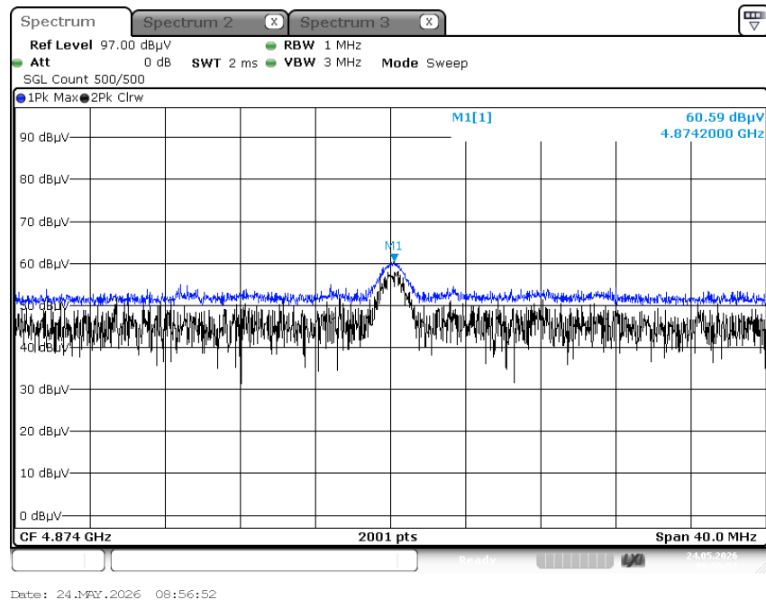
Radiated Spurious Emissions plot – Peak Result (802.11b_1 Mbps, Ch.6 2nd Harmonic, Y-H)
