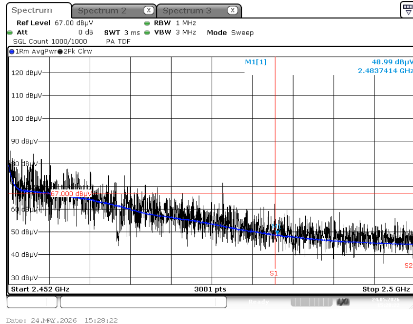
Radiated Restricted Band Edges plot – Average Result (802.11n(HT20)_ MCS0, Ch.7, X-H)
