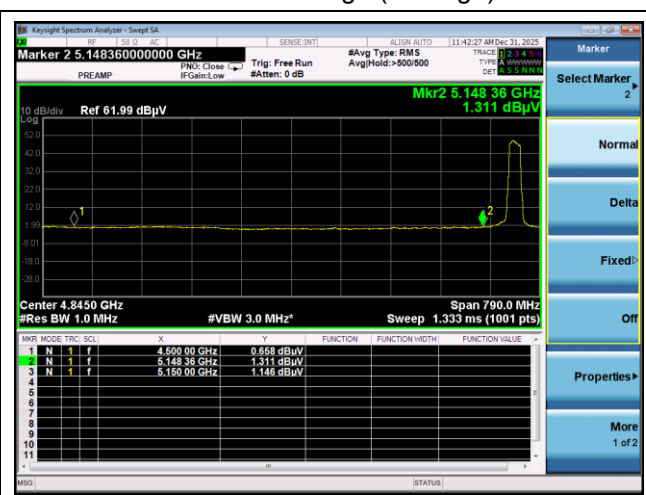
Low channel -1 Band edge (Average) - Band 1
