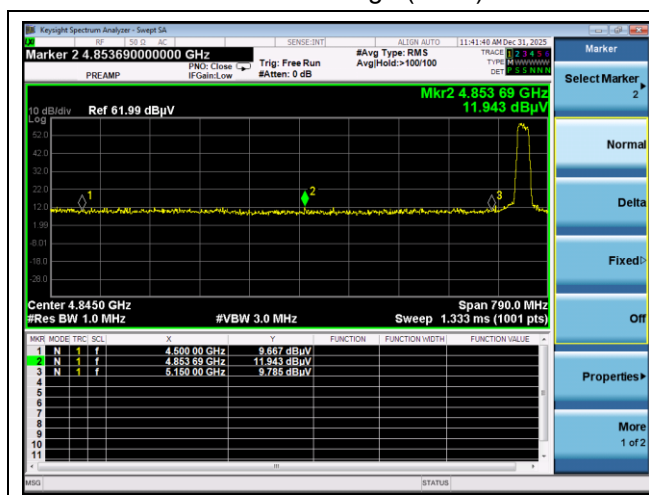
Low channel -1 Band edge (Peak) - Band 1
