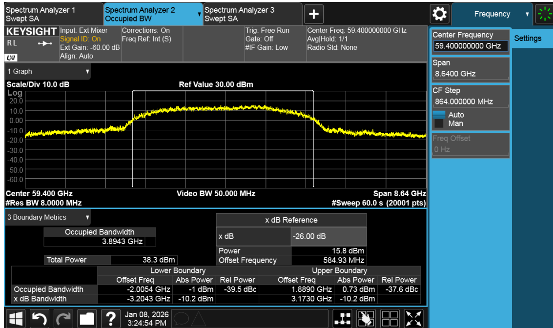
CH.9, Occupied Channel Bandwidth plot (Ant0)
