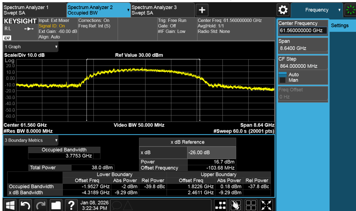
CH.10, Occupied Channel Bandwidth plot (Ant0)
