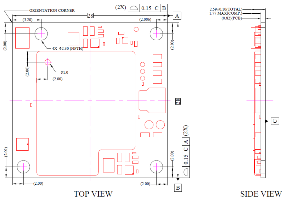
[Figure 5-3] 'LG2851 Box Module' Dimensions
