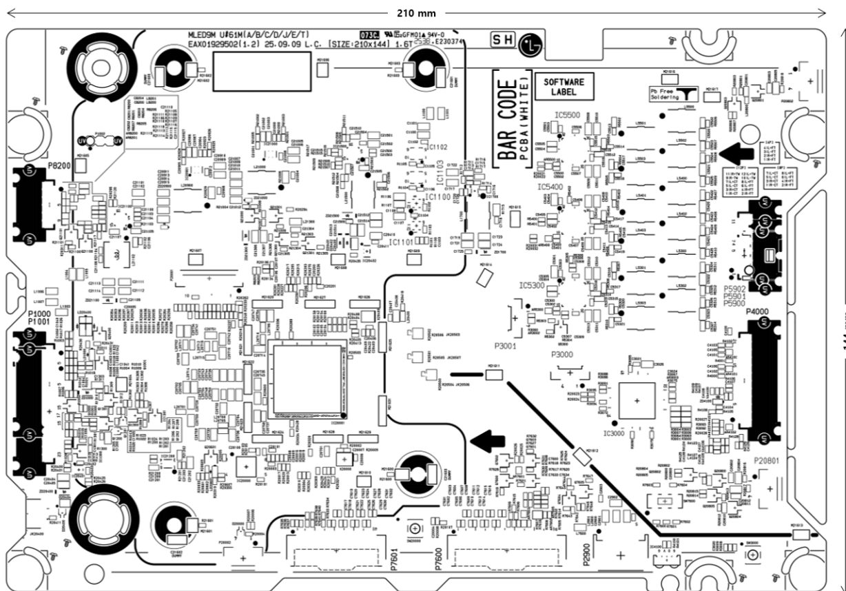
[Figure 5-2] 'LG2832 Display Board' dimensions (Height : 16.0 mm)
