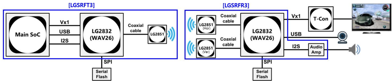
[Figure 1-1] 'LGSRFT3' and 'LGSRFR3' Use Case for 4K 165Hz Wireless TV System
