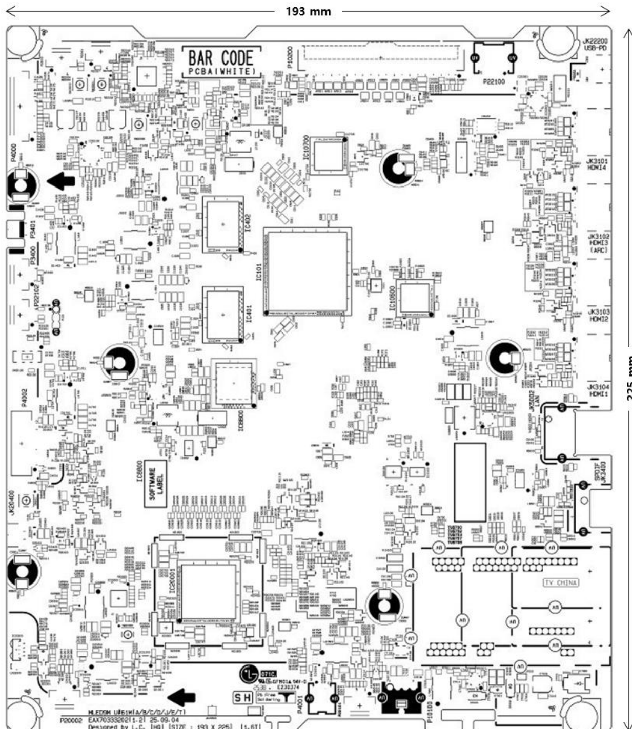
[Figure 5-1] 'LG2832 Box Board' Dimensions (Height : 17.4 mm)
