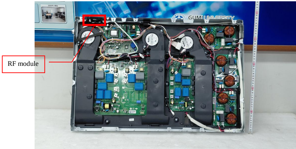
< RF Module Location >
