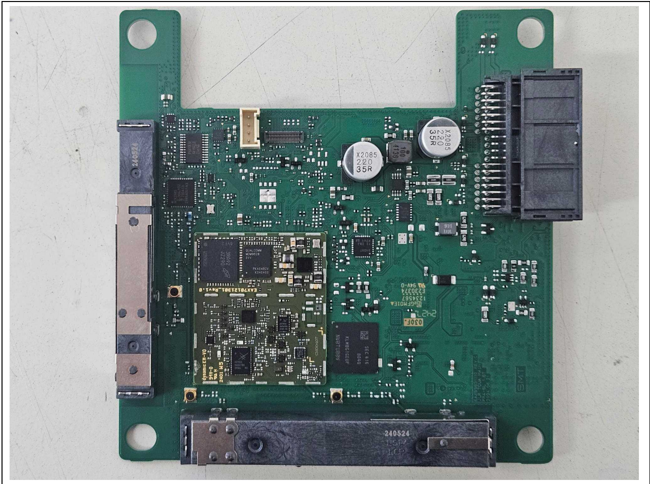
Top view of Main PCB without shield can
