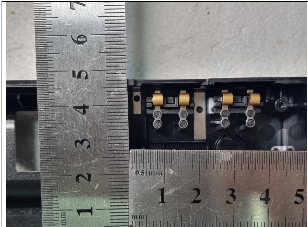
WIFI ANT
