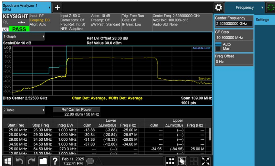
NR7_Low Channel Edge Plot (50 MHz BPSK)-1
