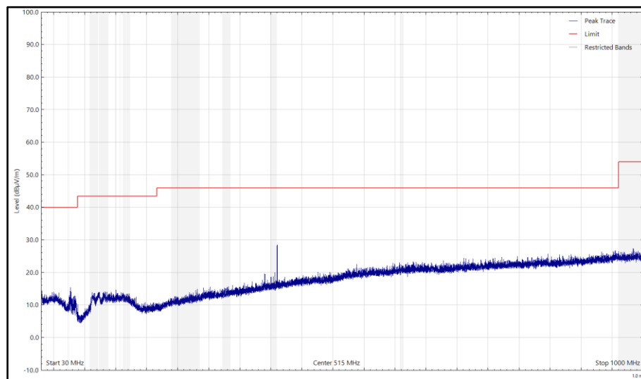
Figure 33 - CH17_LE2M_Y Plane, 2440 MHz, 30 MHz to 1 GHz, Horizontal (Peak)
