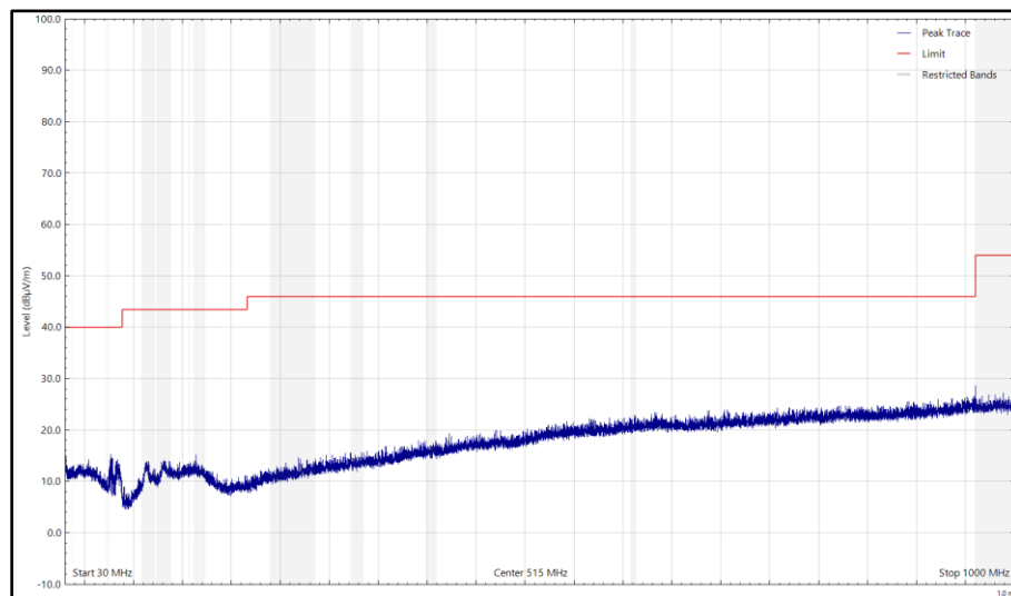
Figure 17 - CH37_LE2M_X Plane, 2402 MHz, 30 MHz to 1 GHz, Horizontal (Peak)
