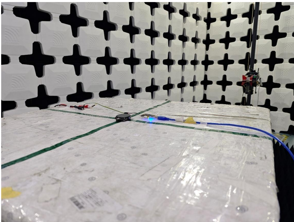
Watch4pro Radiated Emission test Above 1GHz
