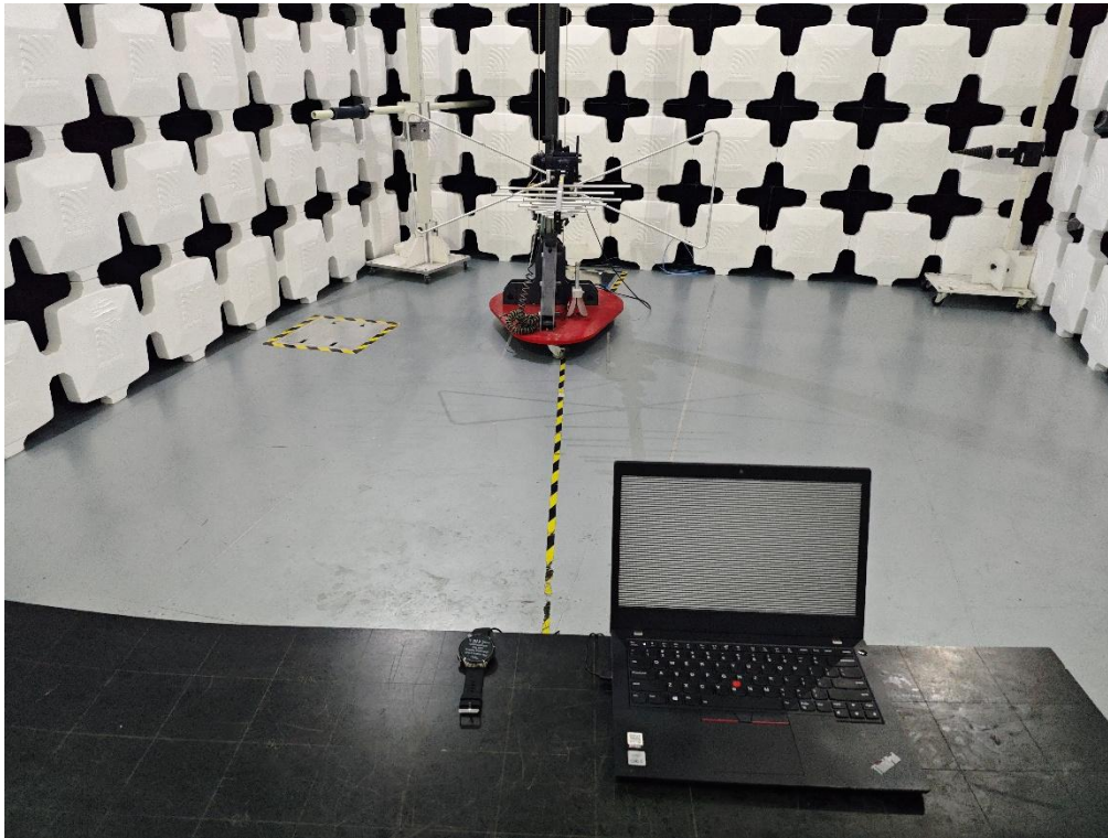
Watch4pro Radiated Emission test below 1GHz
