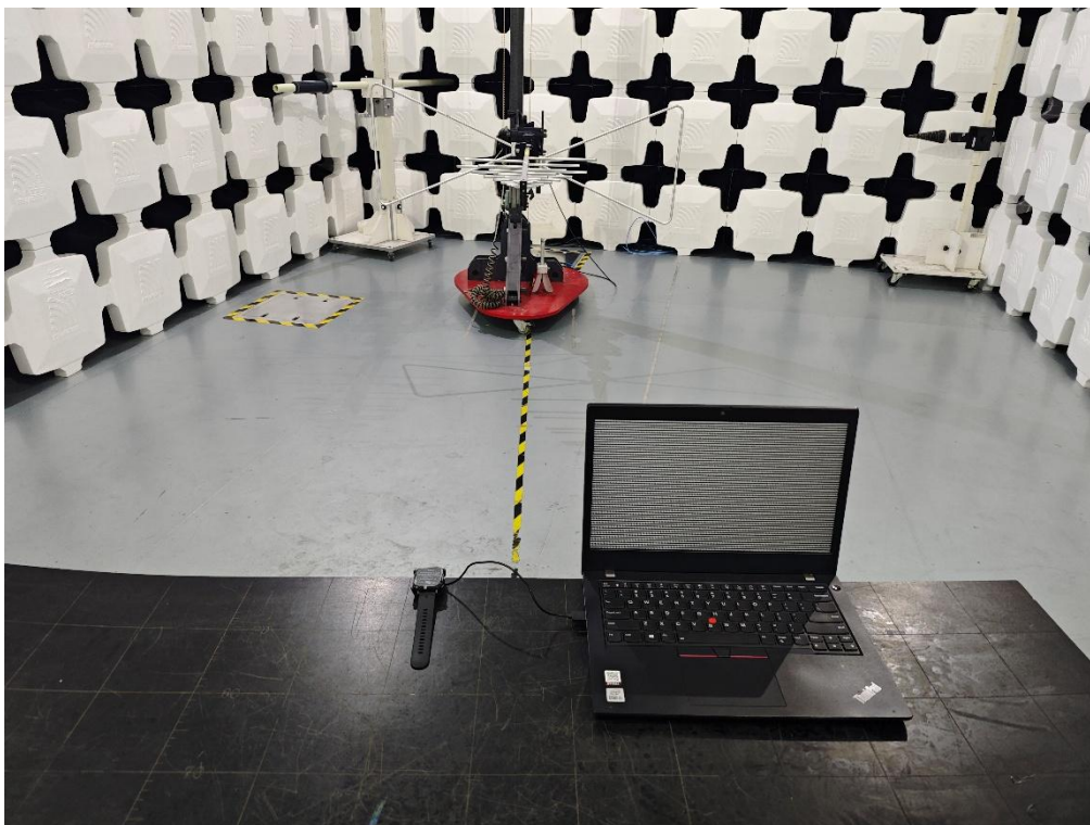
Y13 Radiated Emission test below 1GHz
