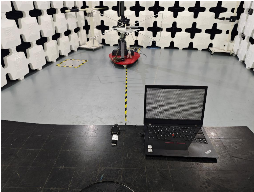
P15 Radiated Emission test below 1GHz
