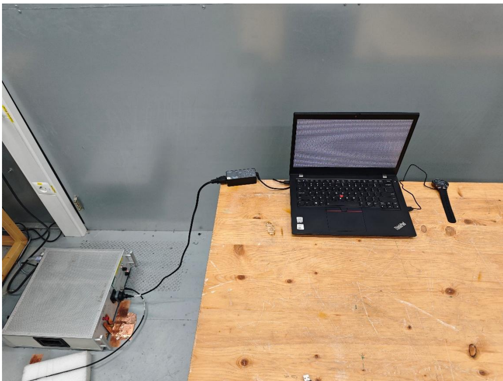
P15 AC line conducted
