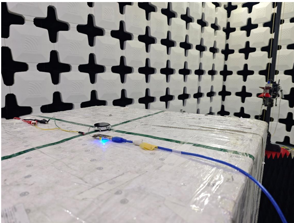
P15 Radiated Emission test Above 1GHz
