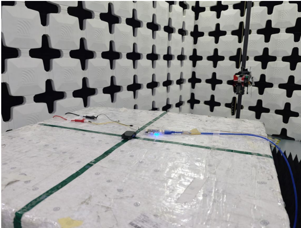
Y13 Radiated Emission test Above 1GHz
