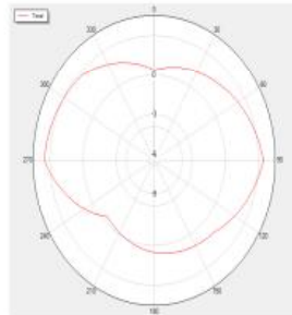
BLUETOOTH_Trp_H39 Total
