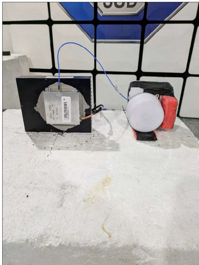
Figure 85 - Radiated Emissions, Z-Plane
