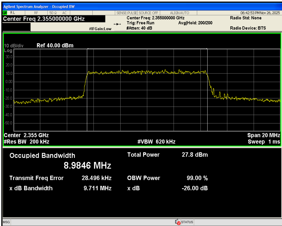
Band40b QAM16 BW=10MHz Channel=39200 RB Size=27 Position=#0
