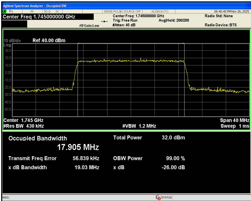
Band66 QAM16 BW=20MHz Channel=132322 RB Size=27 Position=#0
