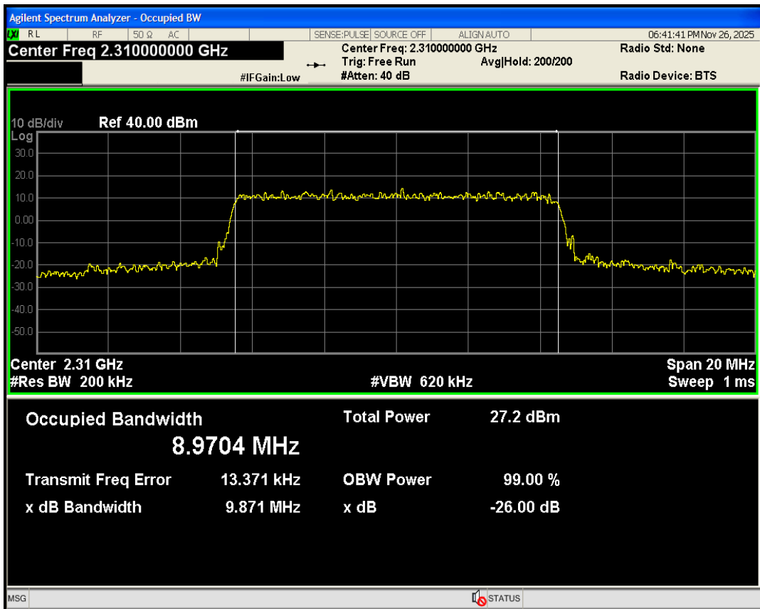
Band40a QAM16 BW=10MHz Channel=38750 RB Size=27 Position=#0
