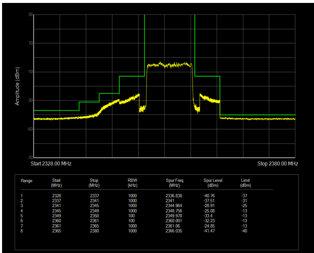
Band40b QAM16 BW=10MHz Channel=39200 RB Size=27 Position=#0
