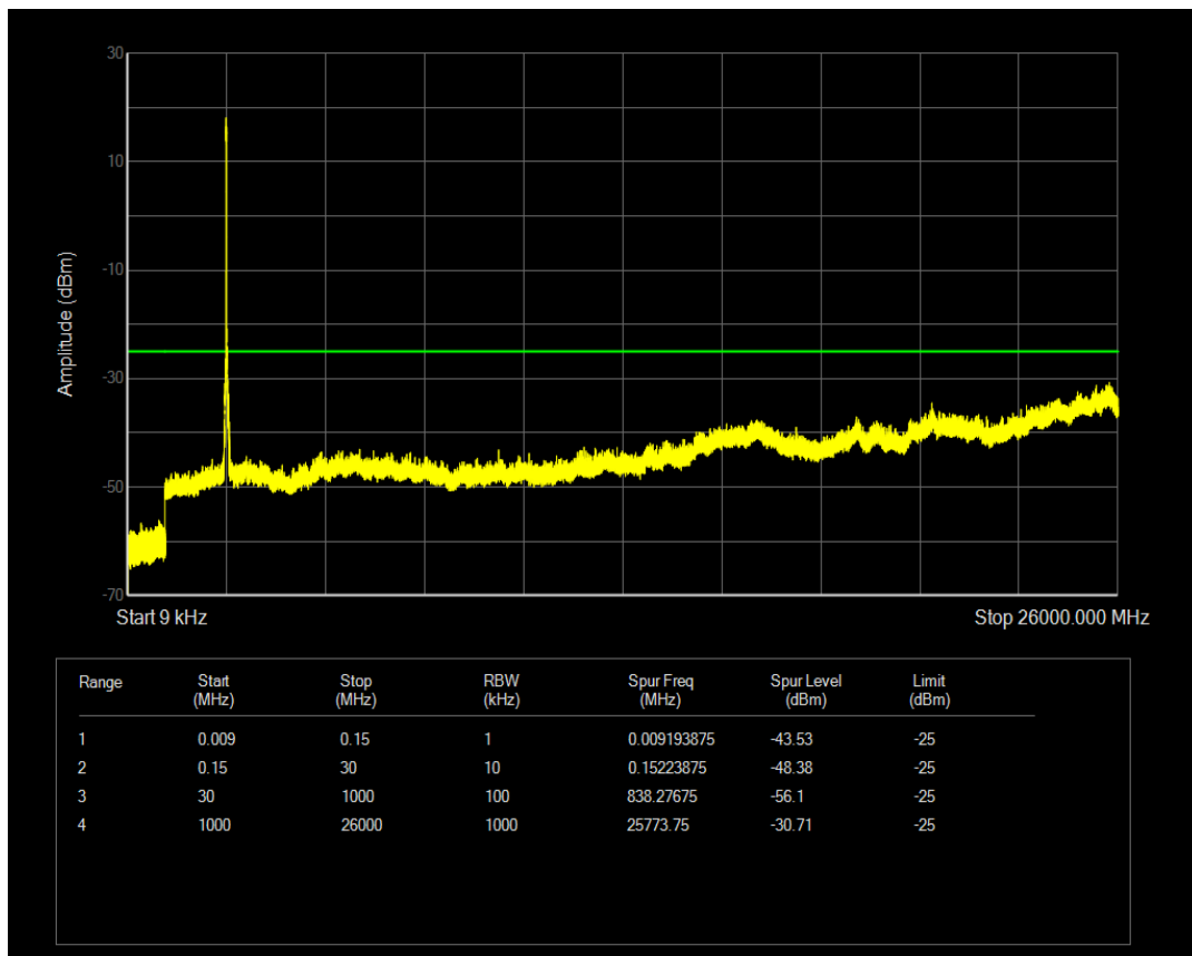
Band38 QAM16 BW=20MHz Channel=38150 RB Size=27 Position=#0
