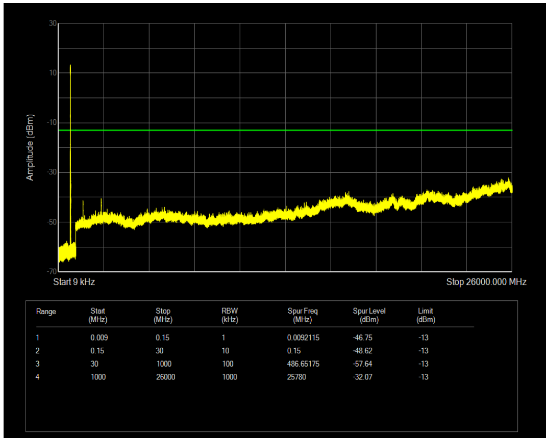
Band17 QAM16 BW=10MHz Channel=23780 RB Size=27 Position=#0
