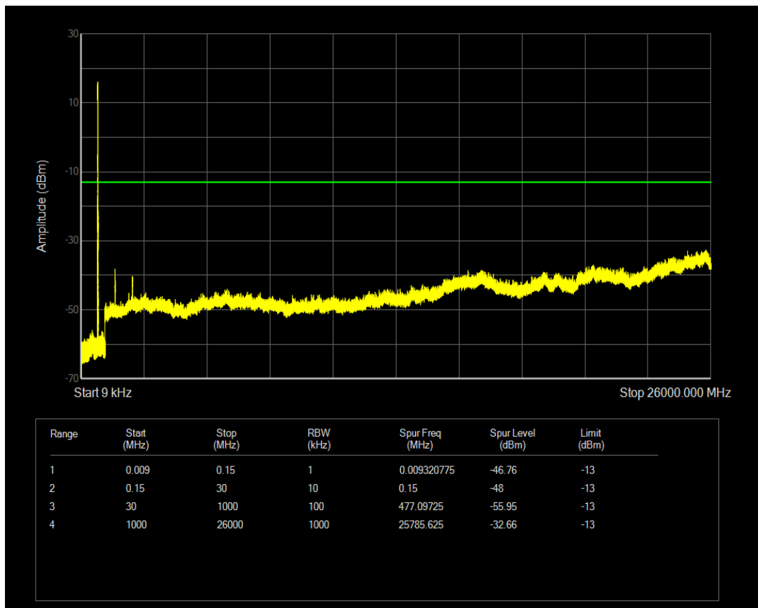
Band17 QAM16 BW=10MHz Channel=23800 RB Size=27 Position=#0
