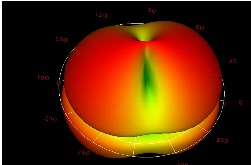
Radiation pattern--2.441GHz
