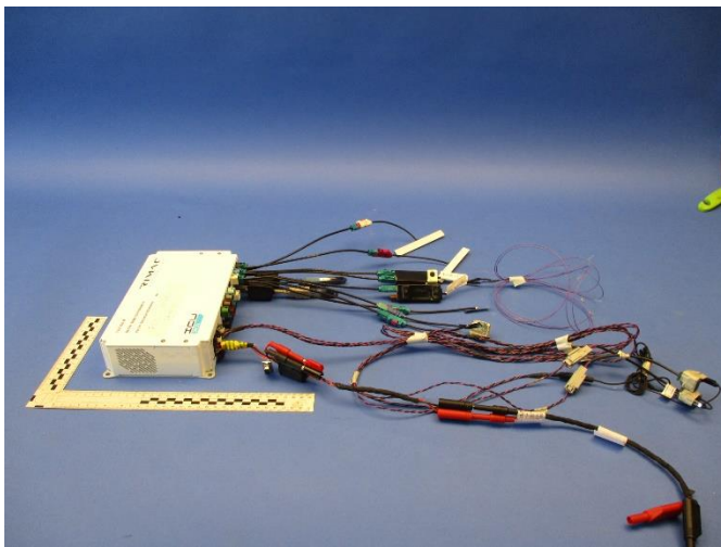
Picture 3 : EUT with accessory cables connected
