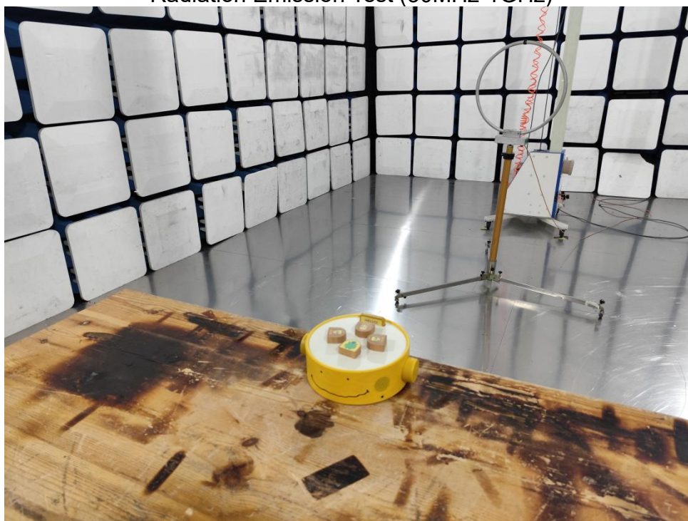
Radiation Emission Test (30MHz-1GHz)
