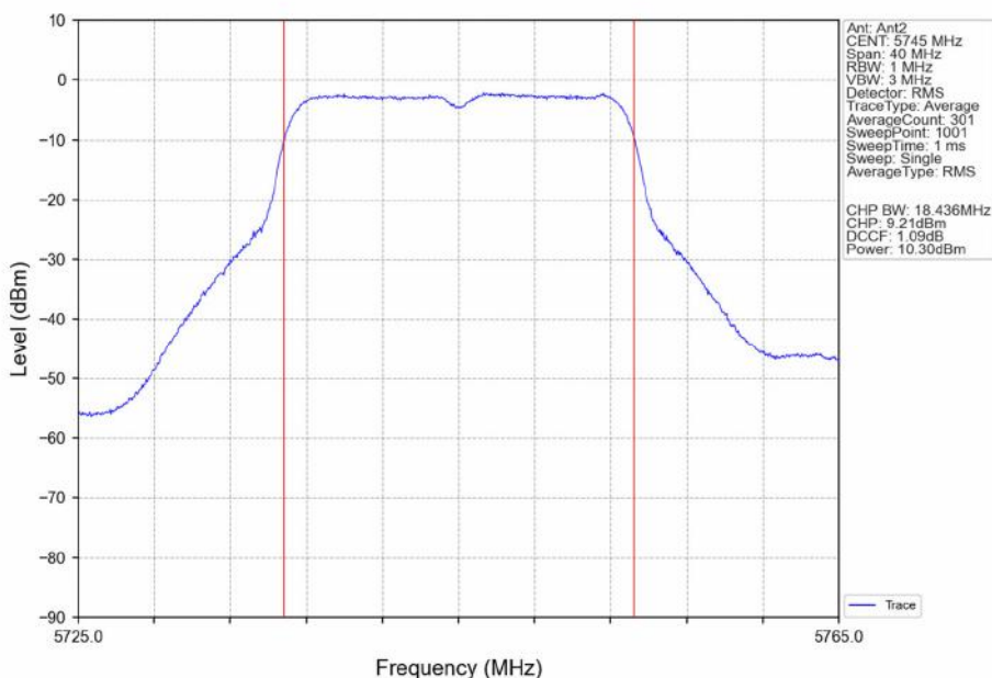
802.11ac(VHT20)_LCH_5745MHz_Ant2_NTNV
