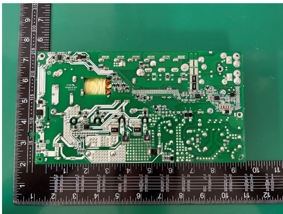
SMPS Board Bottom
