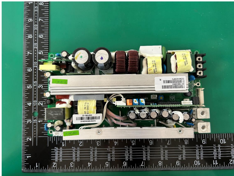
SMPS Board Top
