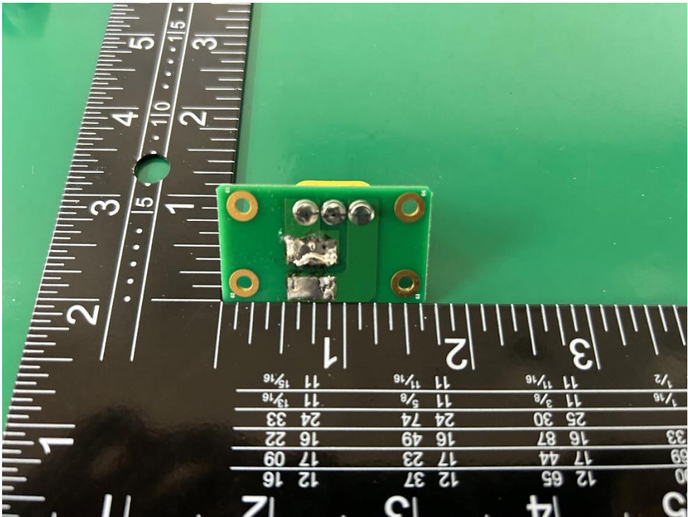
Sub Board Bottom
