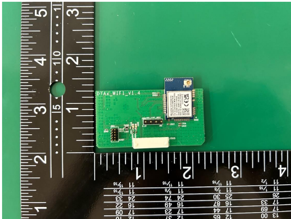
WLAN Board Top
