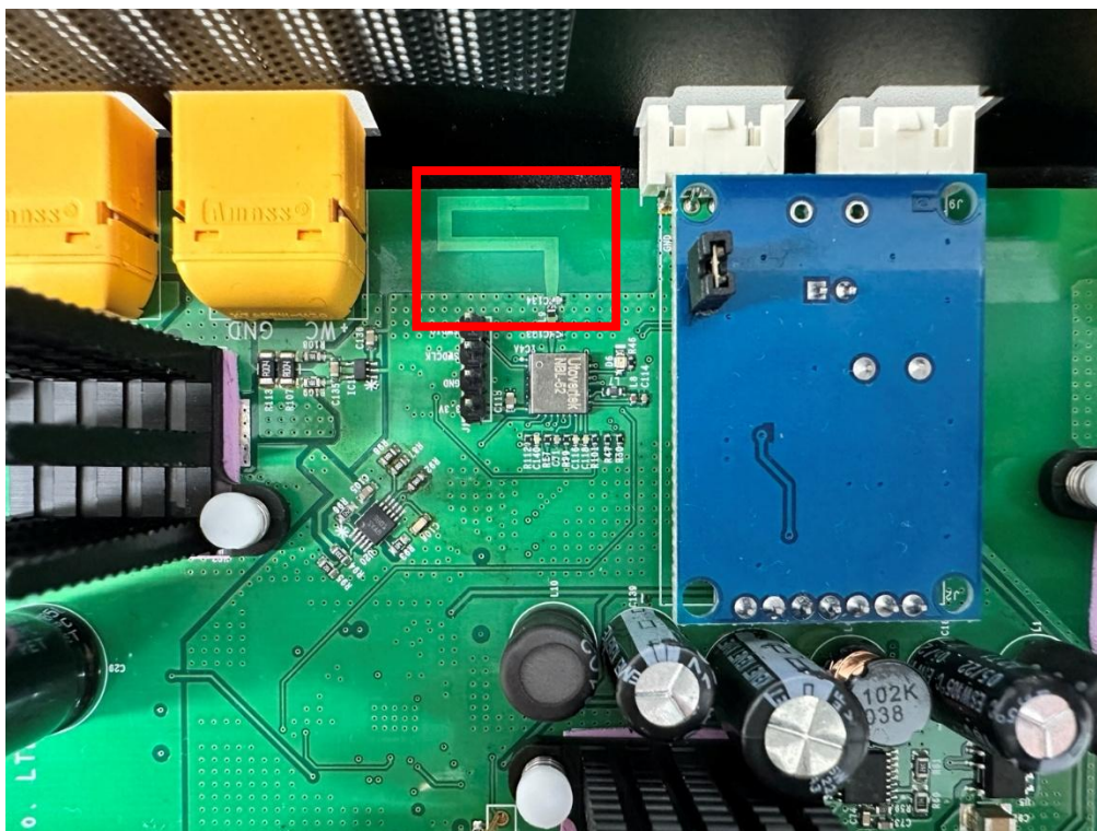
PCB Antenna
