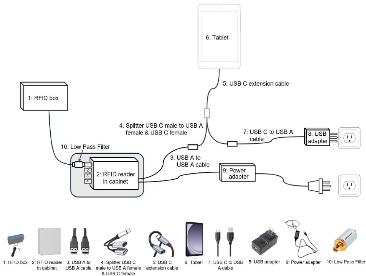
Figure 1 - US RFID box setup
