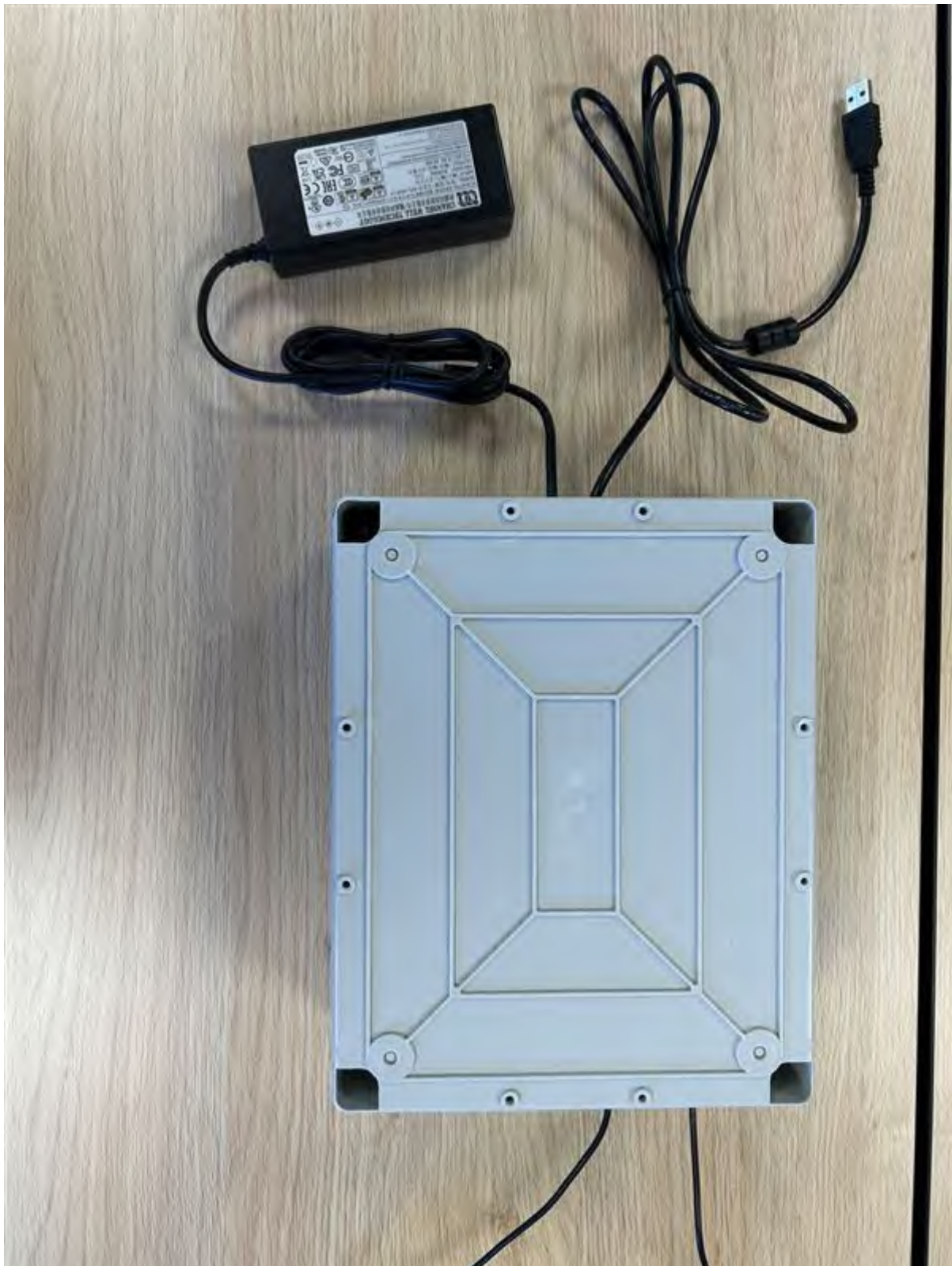
HF RFID Reader RD 2104 BOX Picture from bottom view rev 1.0
