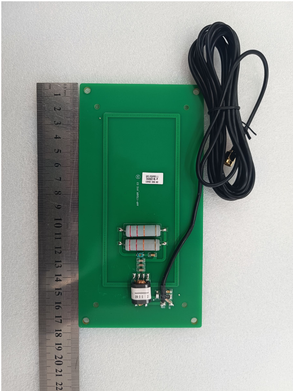
HF RFID Shielded Antenna EA2602-BL-P PCB Picture from top view 1 rev 10.03
