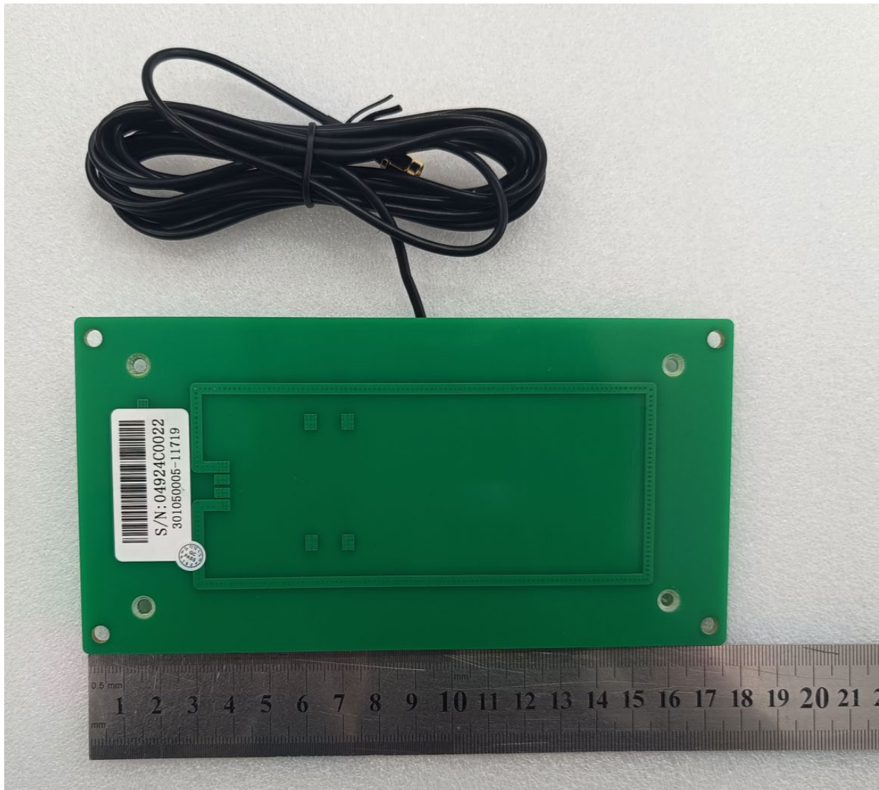
HF RFID Shielded Antenna EA2602-BL-P PCB Picture from bottom view 2 rev 10.03
