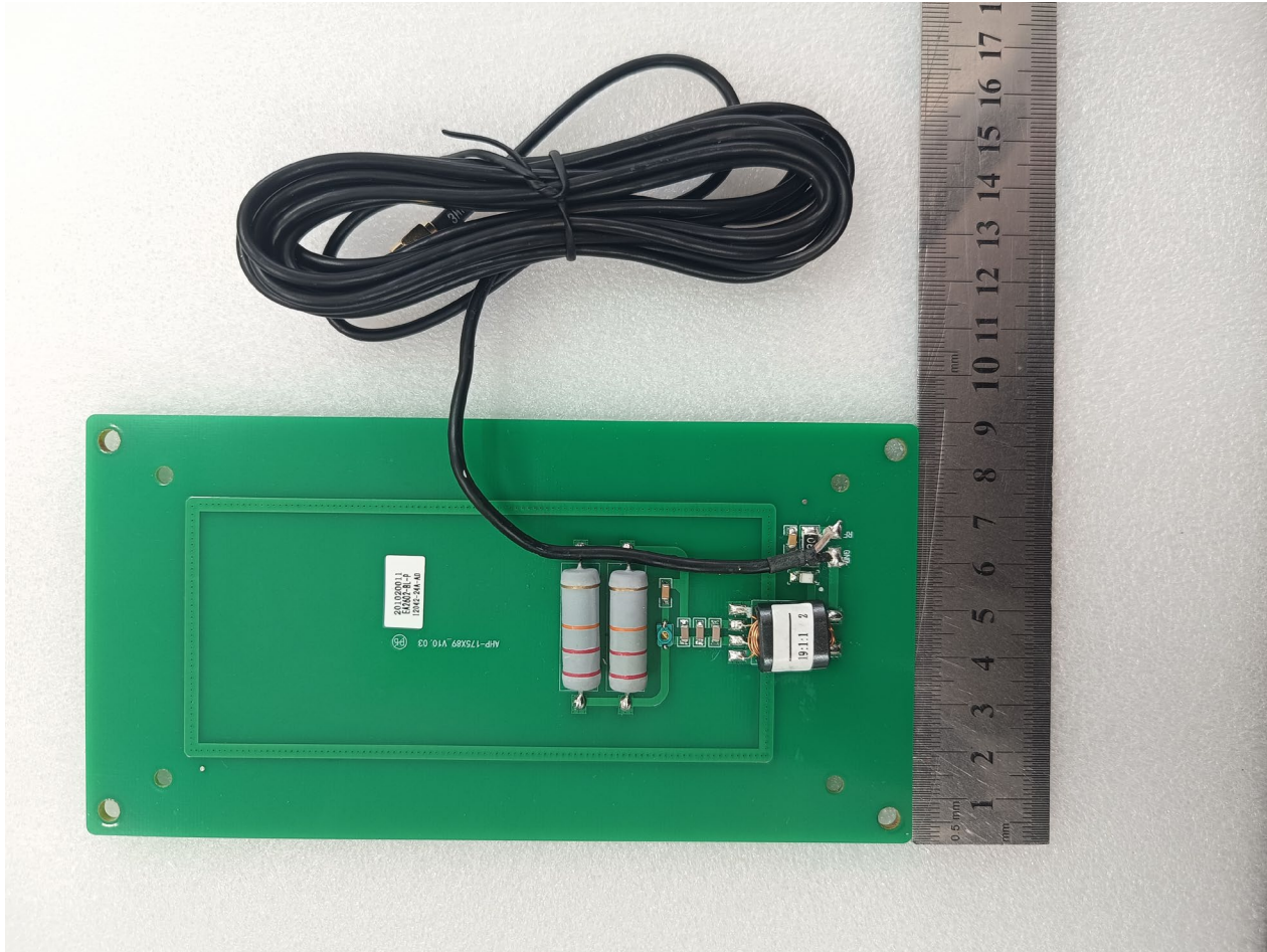
HF RFID Shielded Antenna EA2602-BL-P PCB Picture from top view 2 rev 10.03
