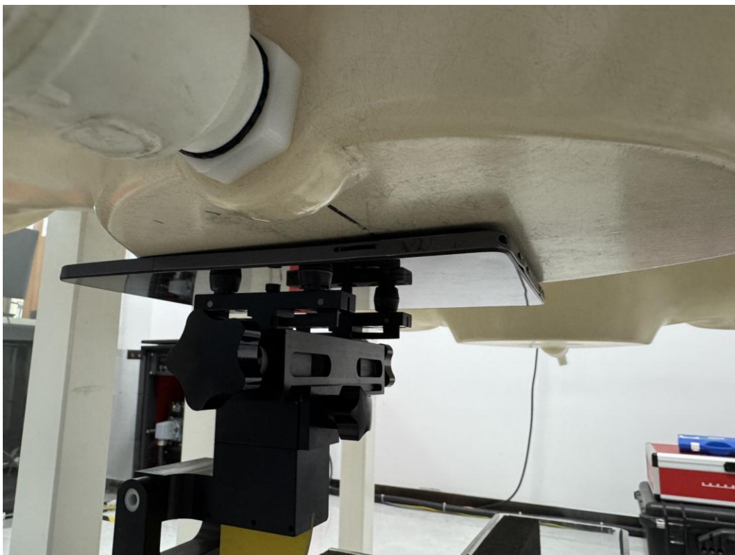
Body Back(WLAN)(0mm)
