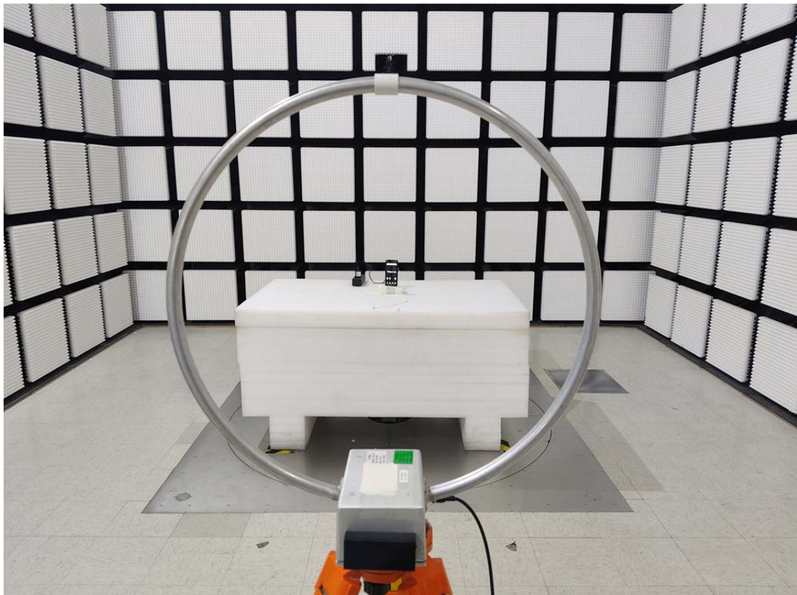
Radiated Emission 9 kHz-30 MHz Parallel View
