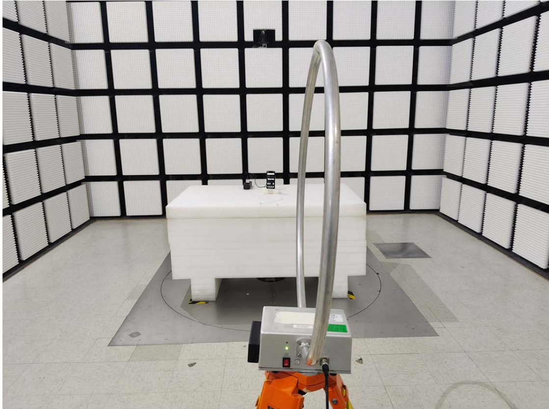
Radiated Emission 9 kHz-30 MHz Perpendicular View
