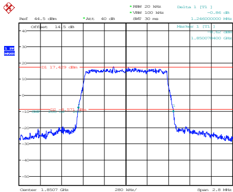
26dB Bandwidth
