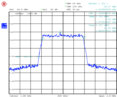
Occupied Bandwidth
