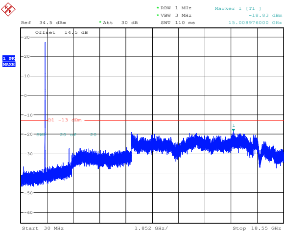
5MHz_Low_QPSK_1@0(30MHz~18.55GHz)
