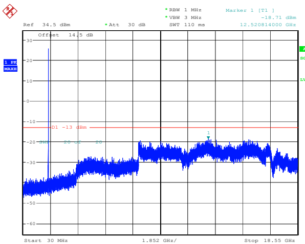
10MHz_Low_QPSK_1@0(30MHz~18.55GHz)
