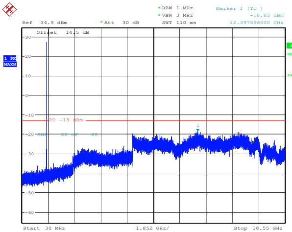
5MHz_Middle_QPSK_1@0(30MHz~18.55GHz)
