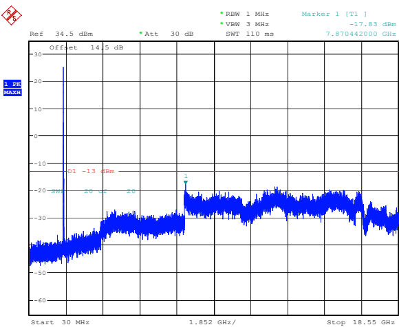
10MHz_Middle_QPSK_1@0(30MHz~18.55GHz)
