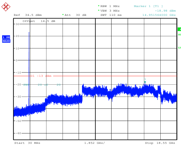
10MHz_High_QPSK_1@0(30MHz~18.55GHz)
