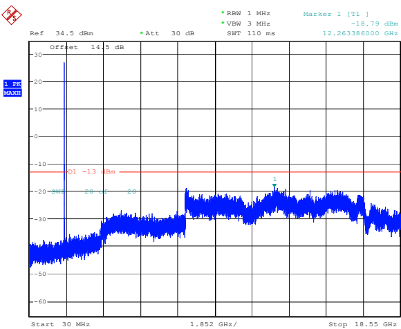
5MHz_High_QPSK_1@0(30MHz~18.55GHz)
