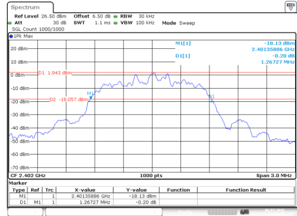
2DH1_Low
