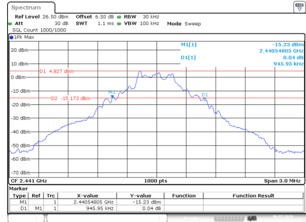
DH1_Middle
