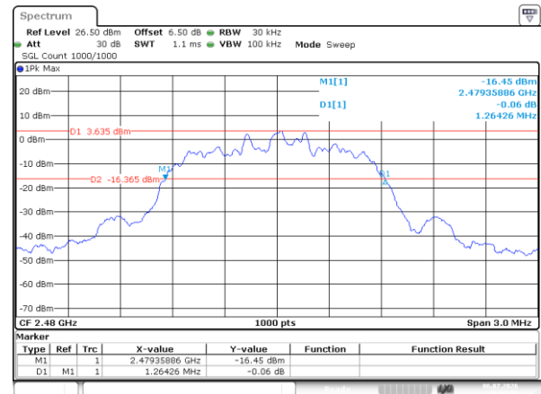
2DH1_High
