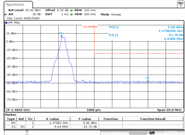
DH1_High
