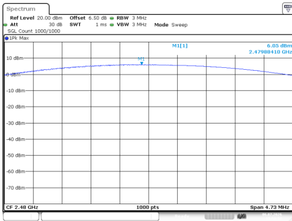
DH1_High
