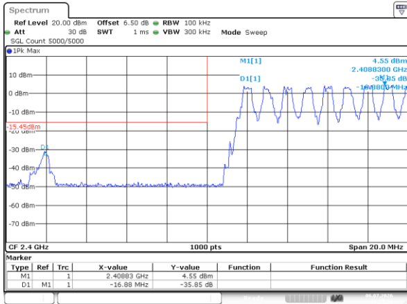
DH1_Hopping_Lower
