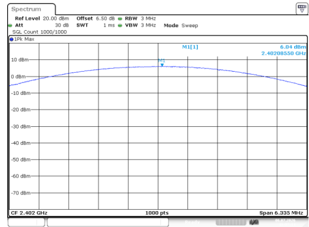
2DH1_Low
