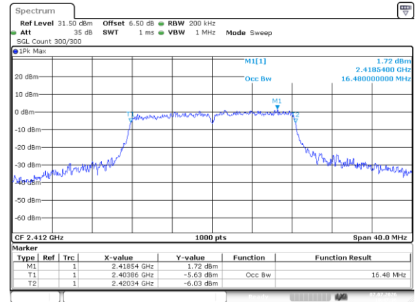
802.11g_2412MHz
