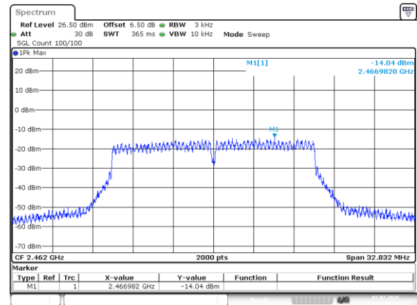
802.11g_2462MHz
