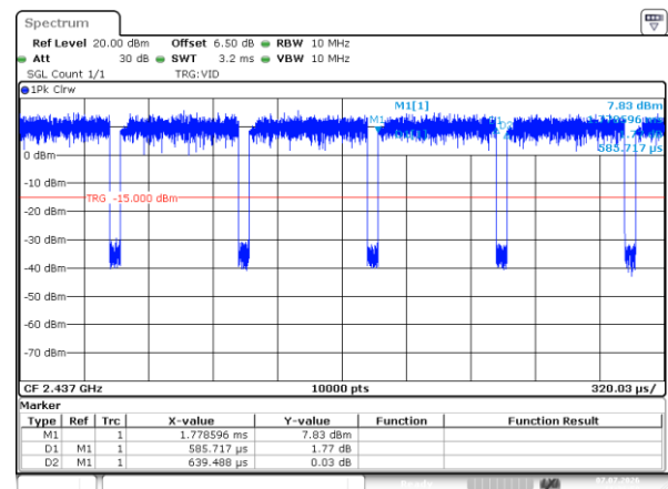
802.11n40_2437MHz
