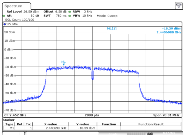
802.11n40_2452MHz
