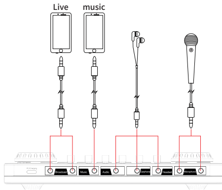
② Live streaming using 3.5 audio cable
