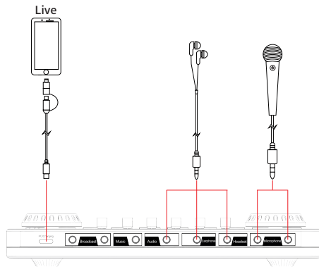
① Live streaming using OTG cable
