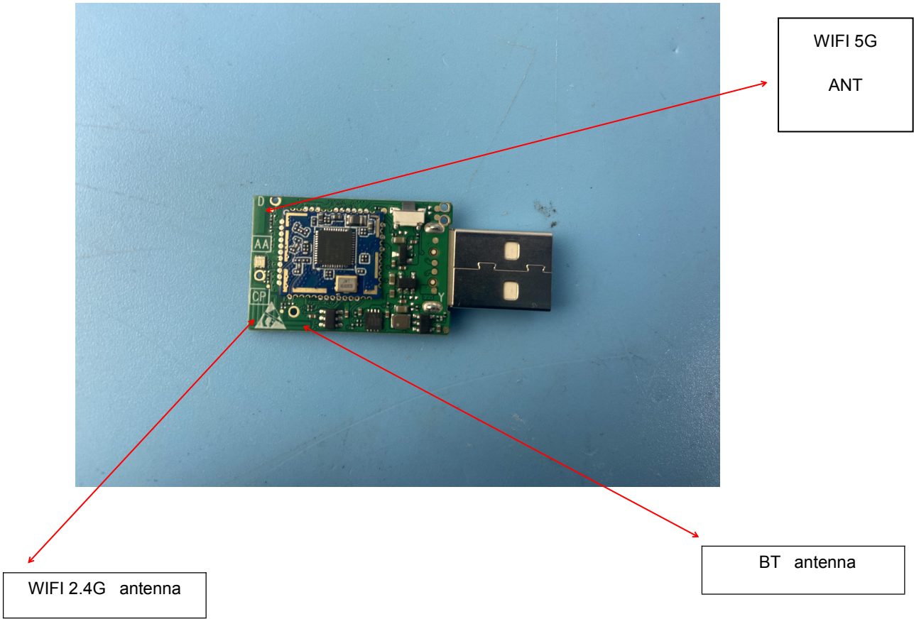
INTERNAL PHOTO OF SAMPLE PCB
