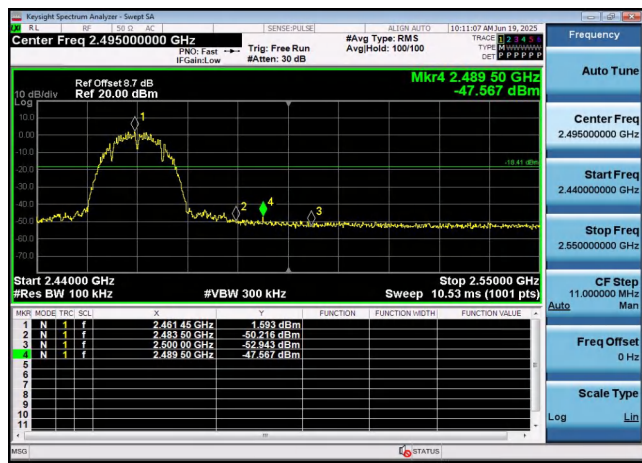
Right bandedge
