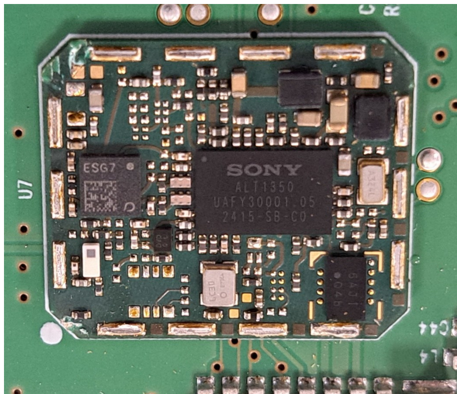
radio module internals
