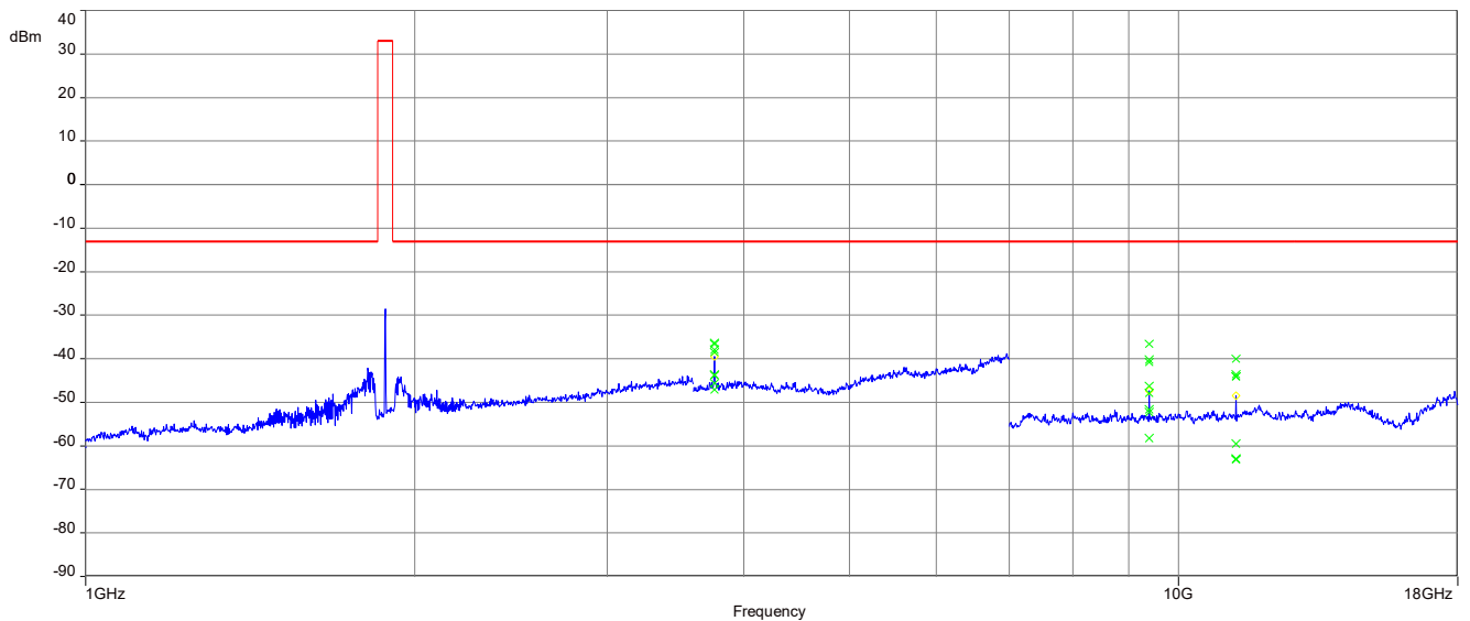
Plot 3: Mid channel (1 GHz – 18 GHz)
