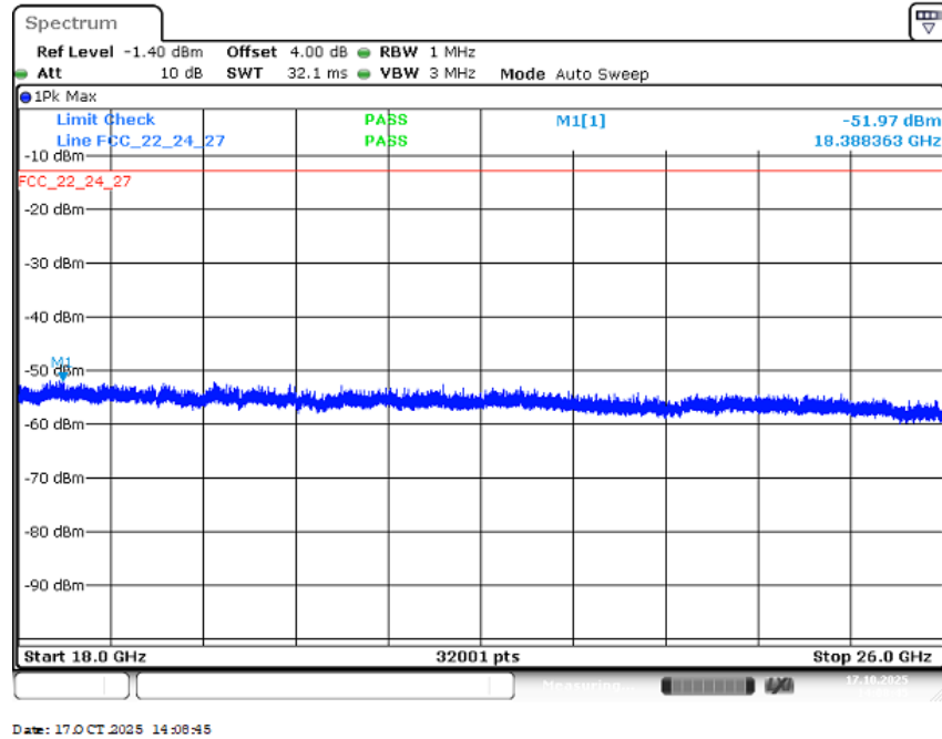
Plot 4: Mid channel (18 GHz – 26 GHz), valid for both modulations
