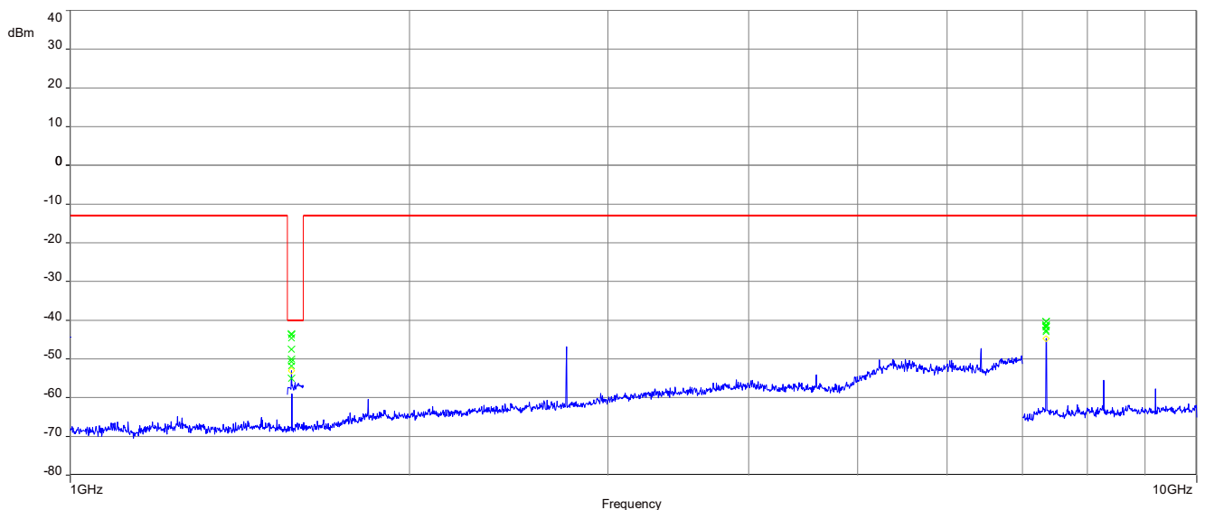
Plot 1: 1 GHz to 10 GHz, vertical & horizontal polarization
