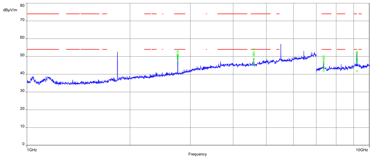
Plot 1: 1 GHz – 10 GHz, horizontal &amp; vertical polarisation 918.9 MHz
