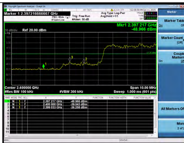
Bluetooth 3DH5
