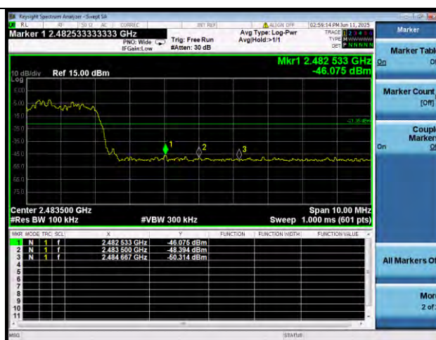
Bluetooth 3DH5
