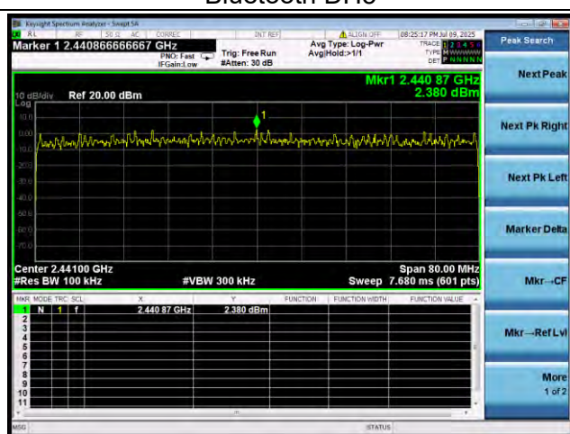
Bluetooth 2DH5
