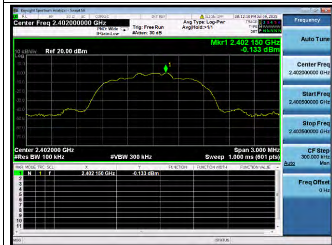
Bluetooth 3DH5 2402MHz
