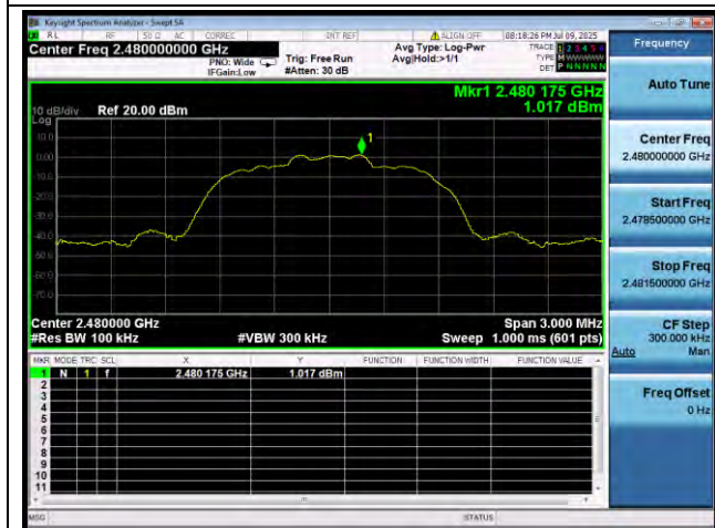
Bluetooth 3DH5 2480MHz
