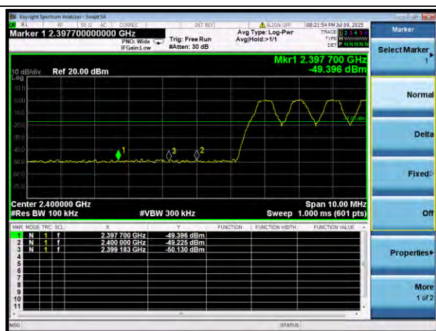
Bluetooth DH5
