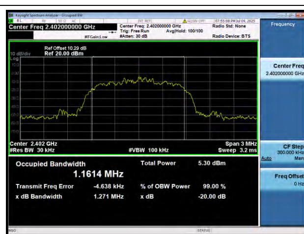
Bluetooth 2DH5 2402MHz
