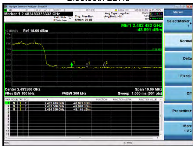
Bluetooth 2DH5
