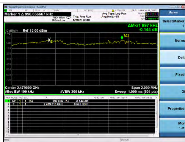
Bluetooth 3DH5 2480MHz
