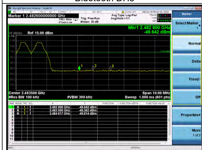
Bluetooth DH5
