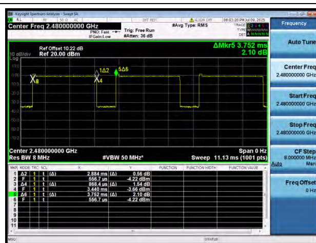
Bluetooth 2DH5 2480MHz
