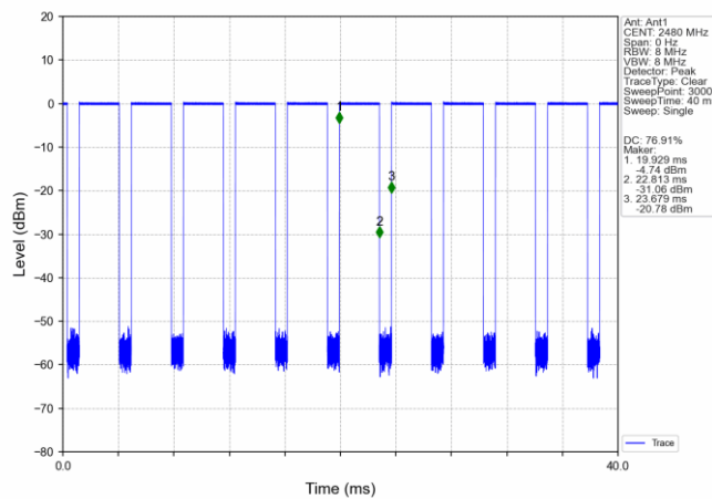
GFSK_DH5_HCH_2480MHz_Ant1_NTNV
