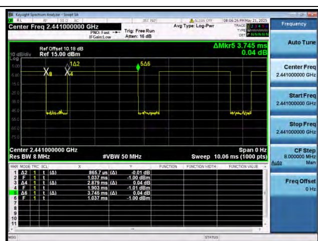
Bluetooth DH5 2441MHz
