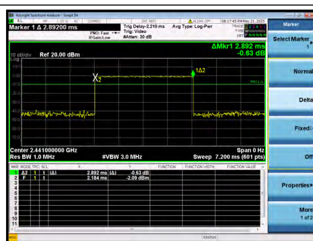
Bluetooth For Classic 2-DH5 2441MHz
