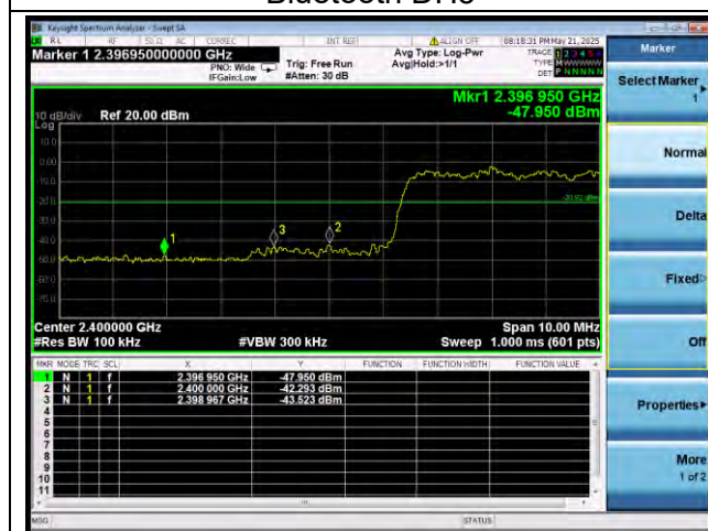
Bluetooth 2DH5
