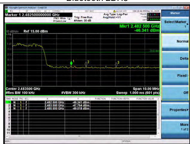
Bluetooth 2DH5
