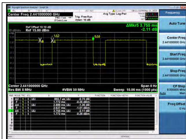
Bluetooth 2DH5 2441MHz
