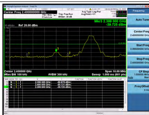
Bluetooth DH5 2402MHz
