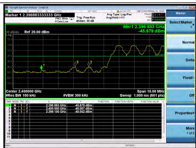
Bluetooth DH5
