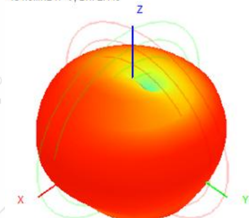
434.0MHz H+V, Eff: 2.1%
