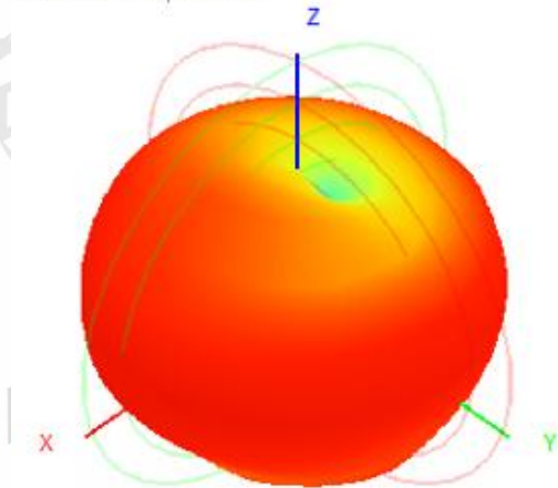
433.0MHz H+V, Eff: 2.1%
