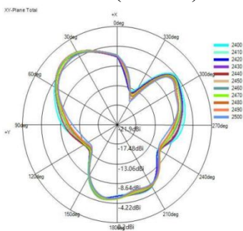
X-Y Plane(unit:dBi):
