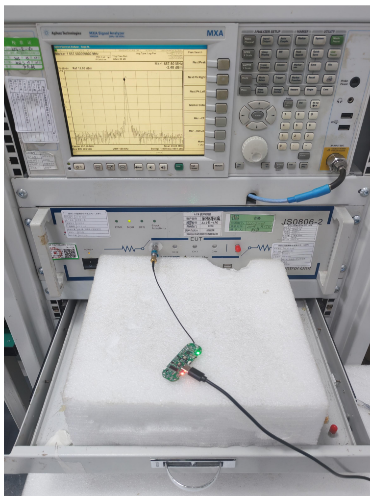
Test Setup Photo(s) of RF Conducted Measurement
