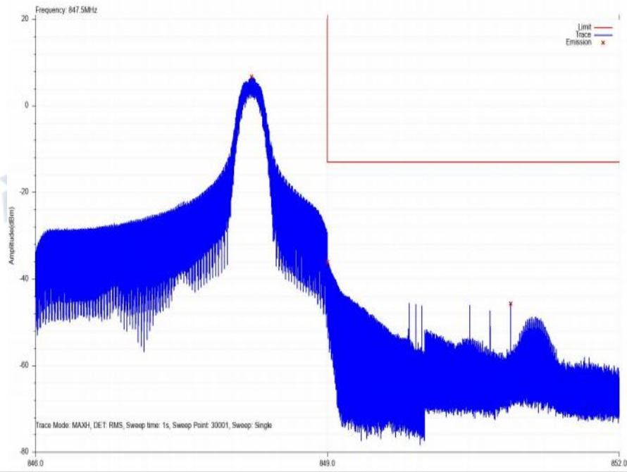
SA_65_NT_NV_0_Band_5_16QAM_3M_CH20635_1_11
