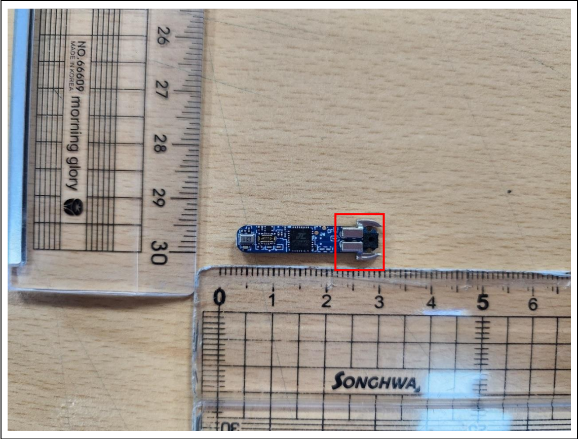
Antenna(2.4GHz ANT)
