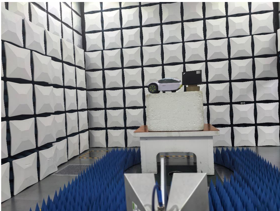
Test Set-up: Radiated spurious emission 1-18GHz
