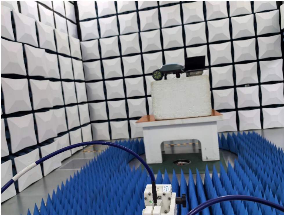
Test Set-up: Radiated spurious emission Above 18GHz
