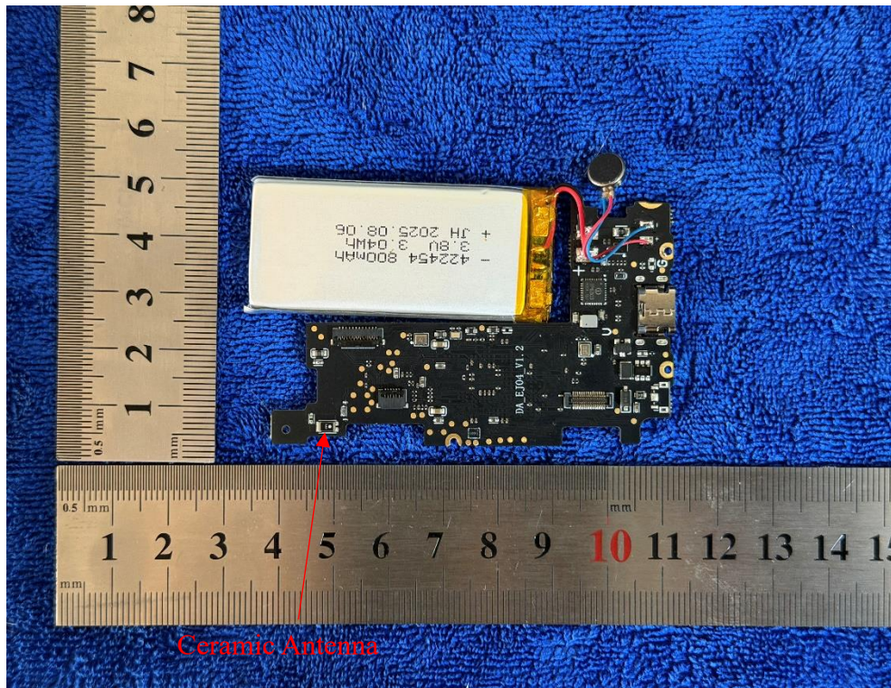
Photo 9: Antenna
