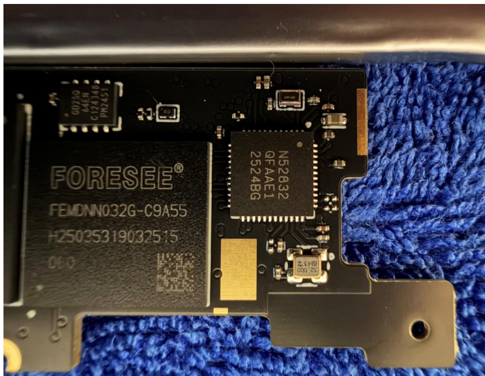
Photo 4: Internal View for PCB
