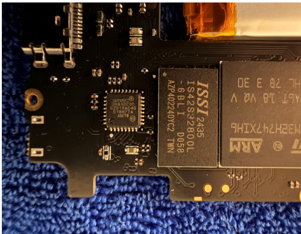
Photo 6: Internal View for PCB
