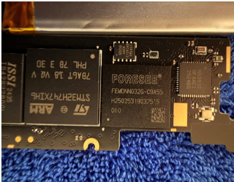
Photo 5: Internal View for PCB
