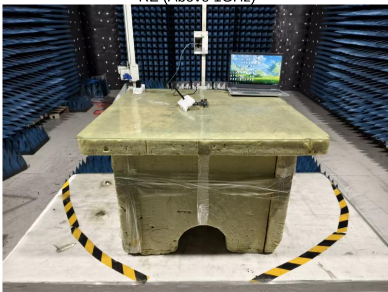
RE (Above 1GHz)
