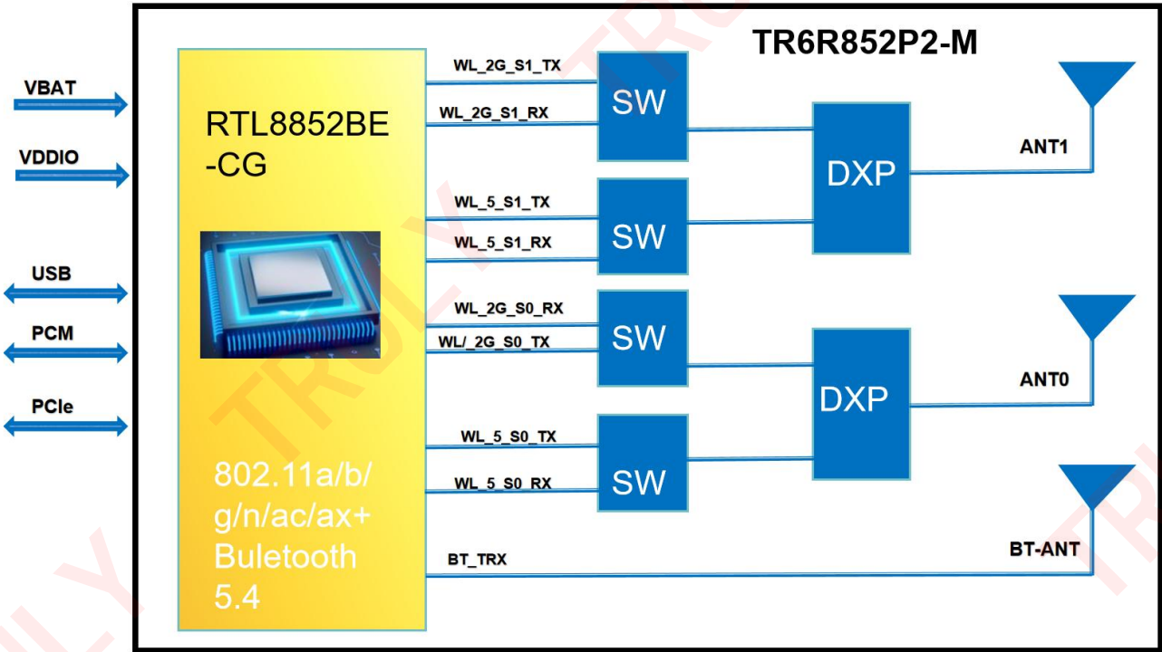
Figure 1. Block Diagram of TR6R852P2-M
