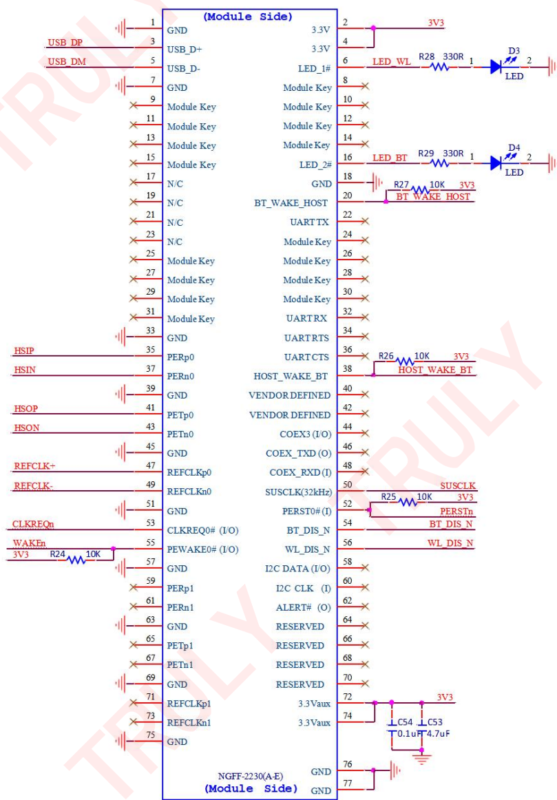
Figure 3. Application Schematic Diagram of TR6R852P2-M
