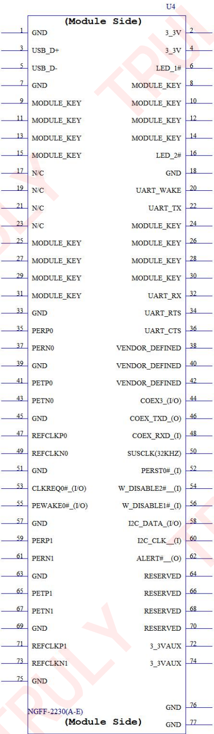
Figure 2.Pin Diagram of TR6R852P2-M
